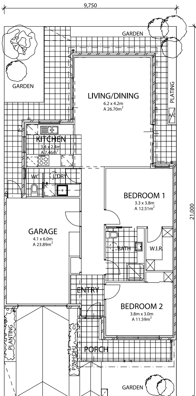
Floor Plan
