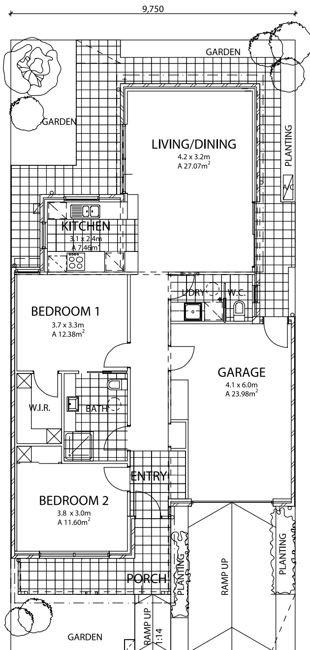
Floor Plan
